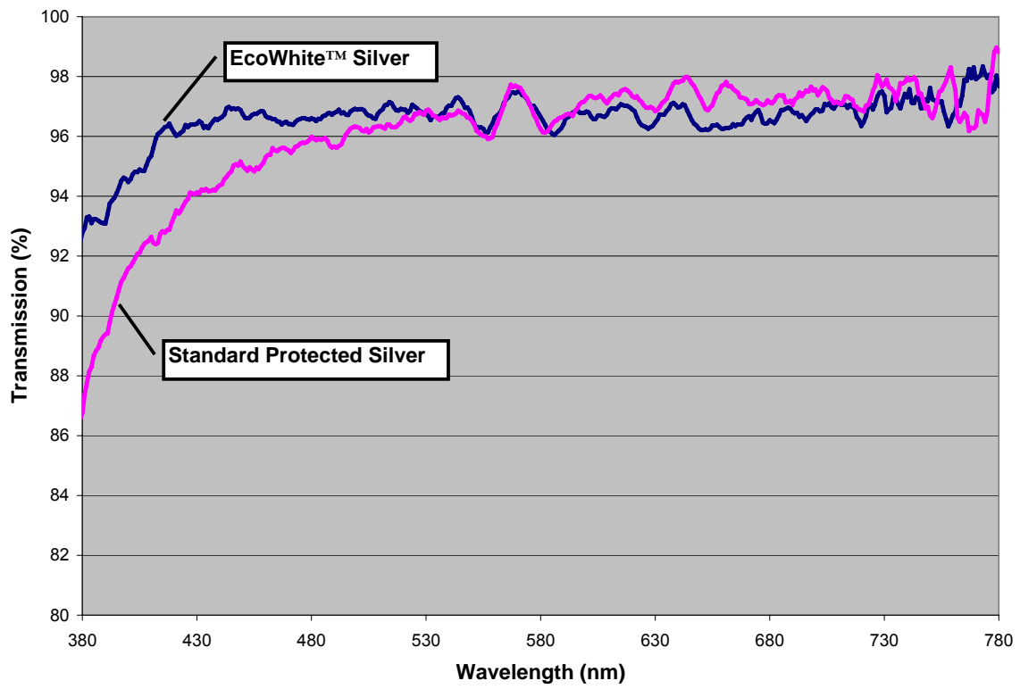
Figure 1 - The reduction in blue roll-off using EcoWhite Silver coatings as compared to the standard protected silver coating saves precious material and results in a “whiter” light.
